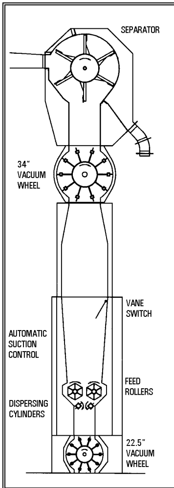
Separator mounted over Automatic Suction Control
