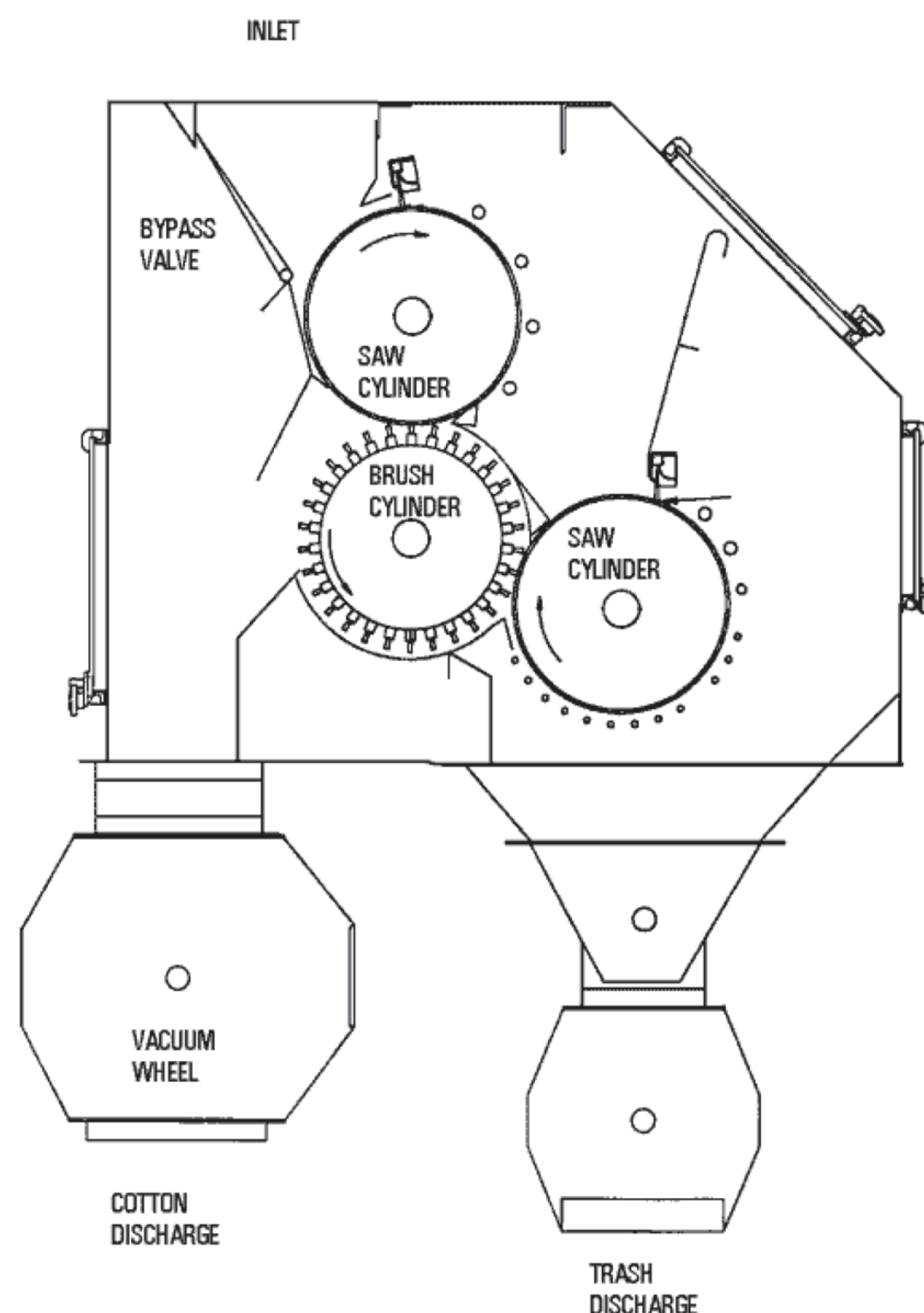
Cross-section of “Little Giant”™ Machine
