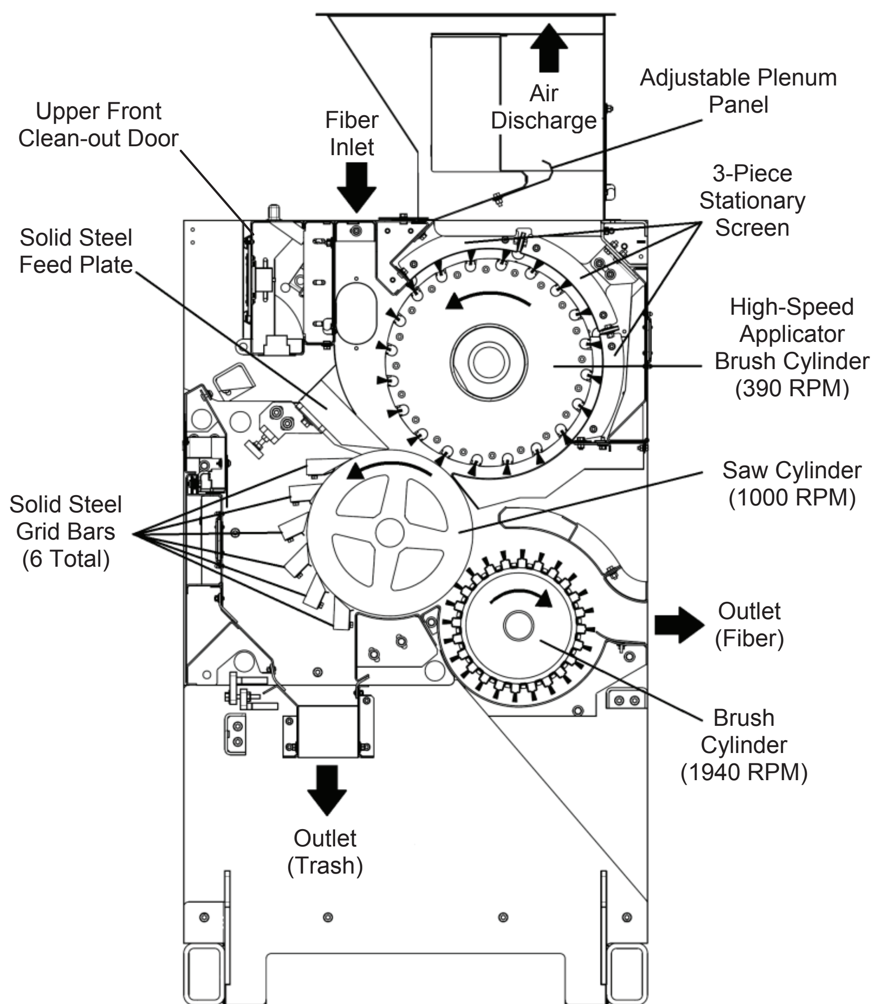
Cross-section of Sentinel™ II Lint Cleaner
