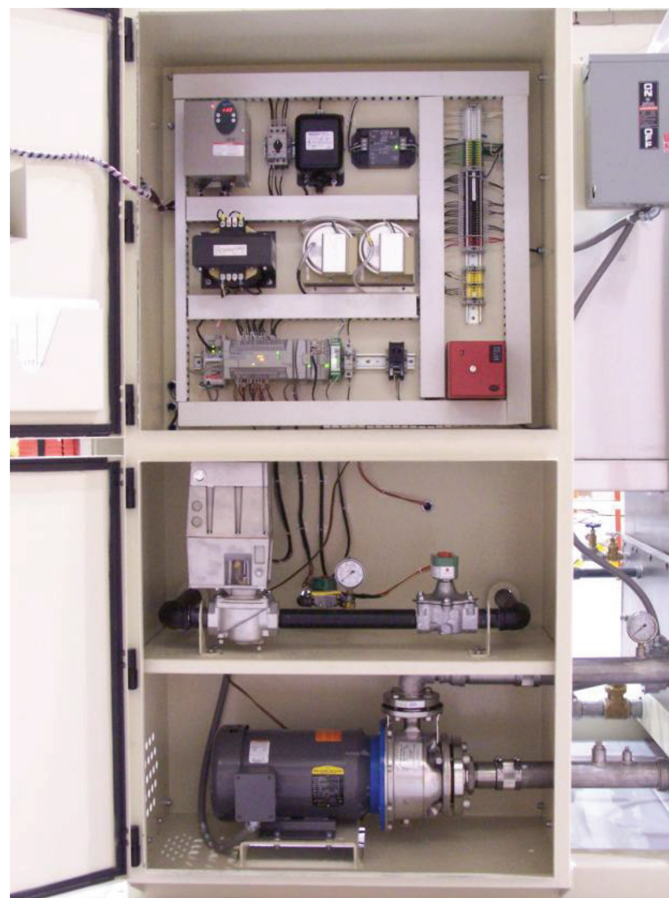
Mist-A-Matic™ Moisture Unit Controls Cabinet Assembly
