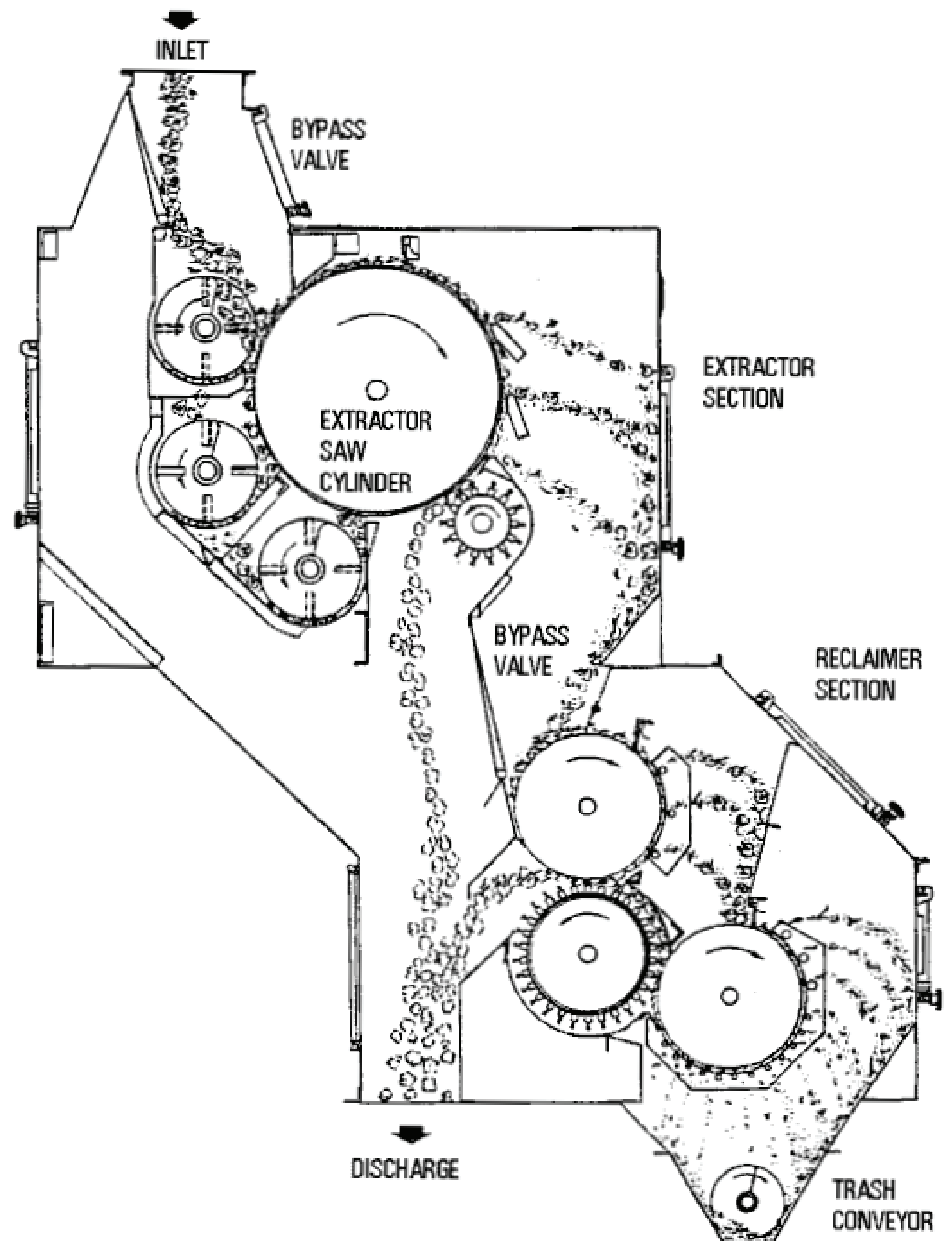
Cross-section of S&GH™ Machine
