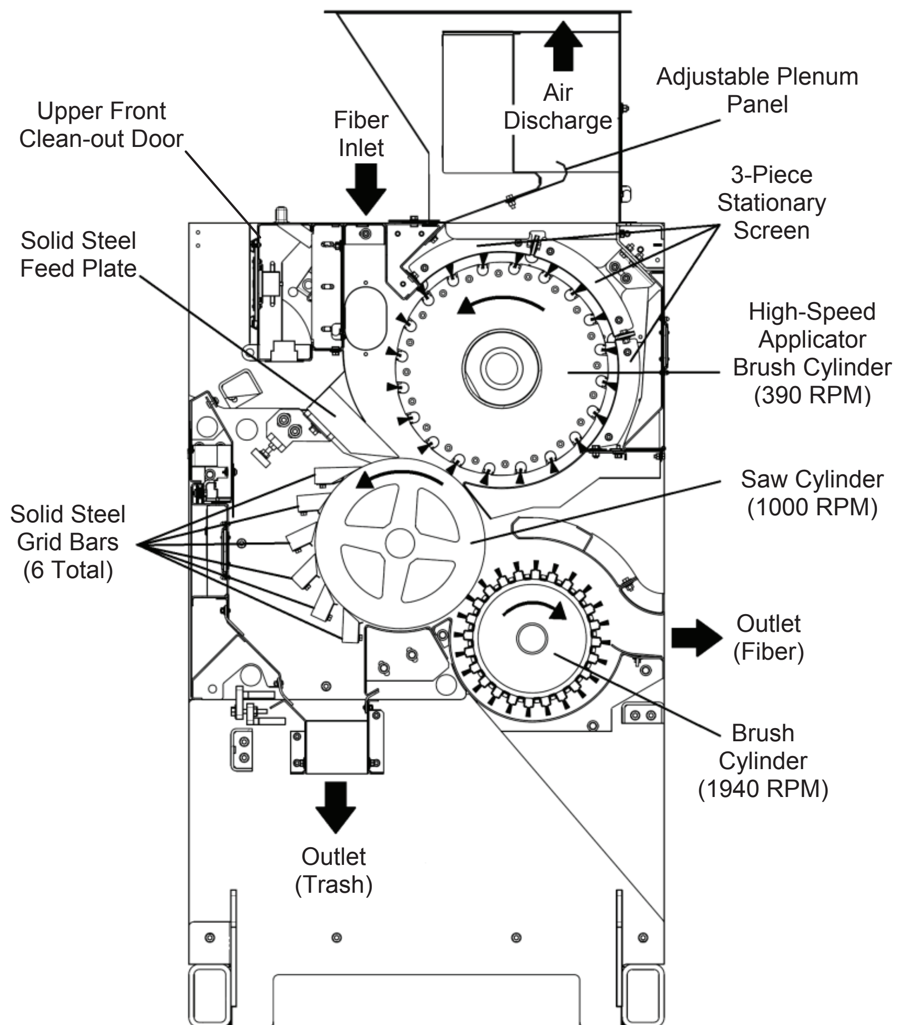
Cross-section of Sentinel™ II Lint Cleaner
