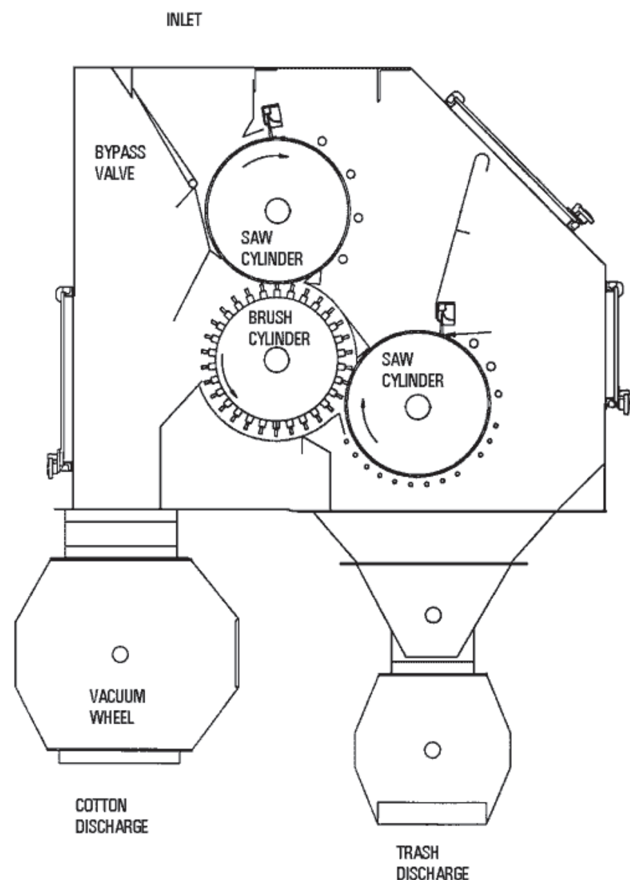
Cross-section of "Little Giant"™ Machine
